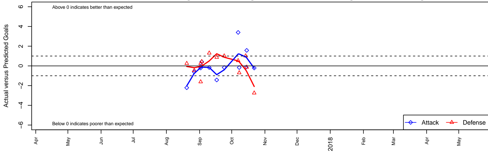
Pumas UNAM B00 Dots are actual minus expected GF (blue circles) and GA (red triangles). Blue line is smoothed change in attack strength. Red is smoothed change in defense strength.
